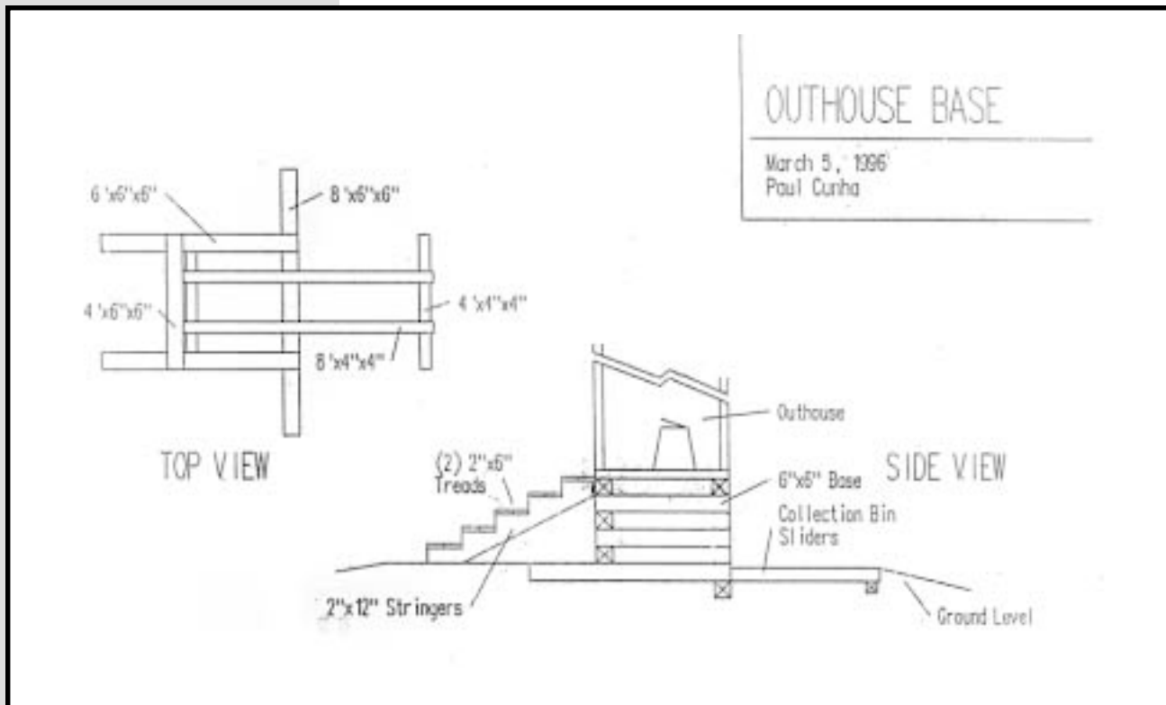
Figure 9.3—This diagram shows how to construct a chamber to house a 70-gallon sewage catcher in either a batch-bin or beyond-the-bin system. This plan is particularly useful for converting an existing outhouse. However, a new outhouse can accommodate a 70-gallon catcher without an elevated foundation requiring a ramp or stairs.” Plans from Paul Cunha and the Appalachian Mountain Club Trails Department.
