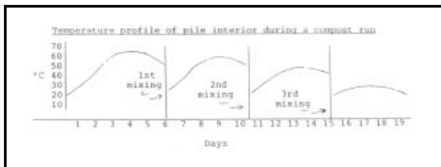
Figure 9.5—Temperature profile of compost pile in a batch-bin system during a compost run.” From the Green Mountain Club.
