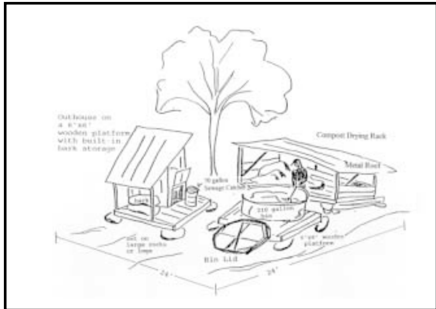
Figure 9.1—Diagram of Green Mountain Club batch-bin composting toilet systems depicting all of the system's components. Note that the outhouse design depicted is only one of several options. Not shown are the two 32-gallon storage cans the Green Mountain Club uses as part of their system. The Appalachian Mountain Club uses two 150-gallon stainless steel composting bins instead of storage cans." Diagram from the Green Mountain Club.
