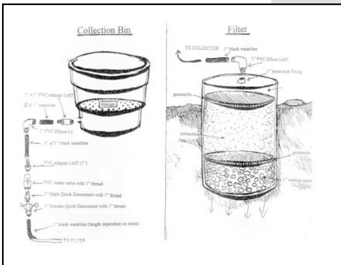
Figure 10.1—The beyond-the-bin liquid management system designed by the Appalachian Mountain Club's Trails Department. This system is an improvement to the Green Mountain Club and Appalachian Mountain Club batch-bin system. Not shown in this diagram is a second barrel that can be attached beyond filter barrel to store filtered effluent. This allows the system to be located near water or in places where drainage is poor. Treated effluent drains into the storage barrel, and is transported to a site with better characteristics for disposal in the ground." Diagram from the Appalachian Mountain Club Trails Dept.
