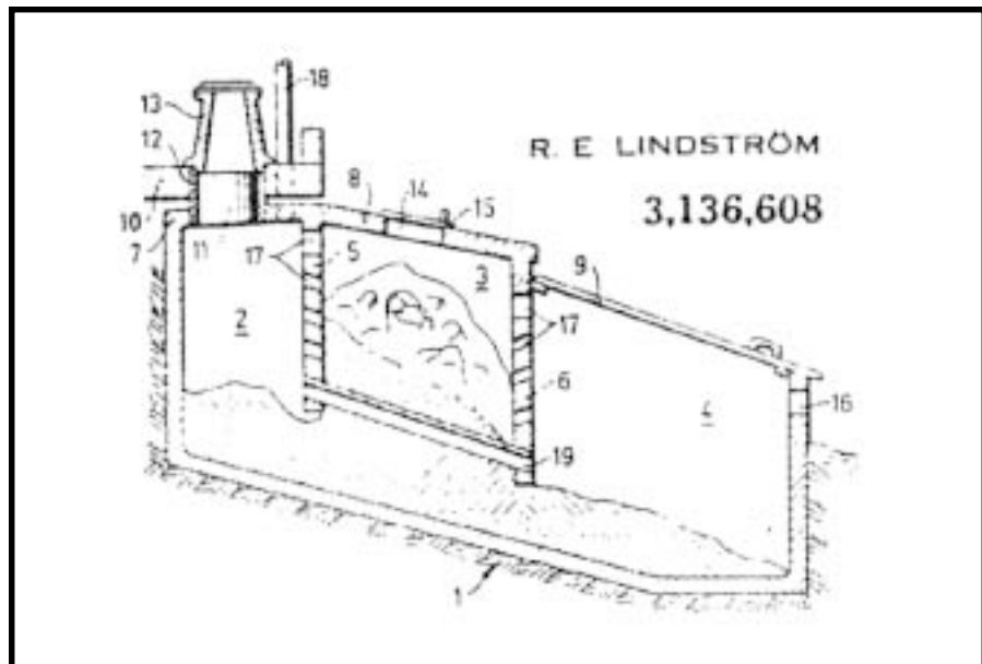
Figure 1.1—Original Clivus Multrum Toilet designed by R.E. Lindstrom of Sweden in the 1930s. Drawing From Stop the Five Gallon Flush (1980) taken from The Composting Toilet System Book by David Del Porto and Carol Steinfeld.
