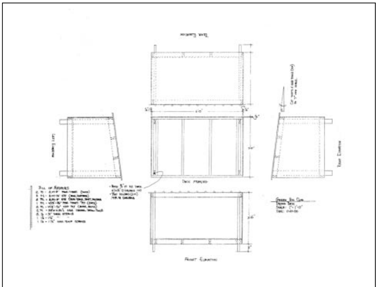
Figure J.1—Diagram of the Green Mountain Club's drying rack, used with their batch-bin and beyond-the-bin and moldering privy systems.” Diagram from Eric Seidel and the Green Mountain Club.
