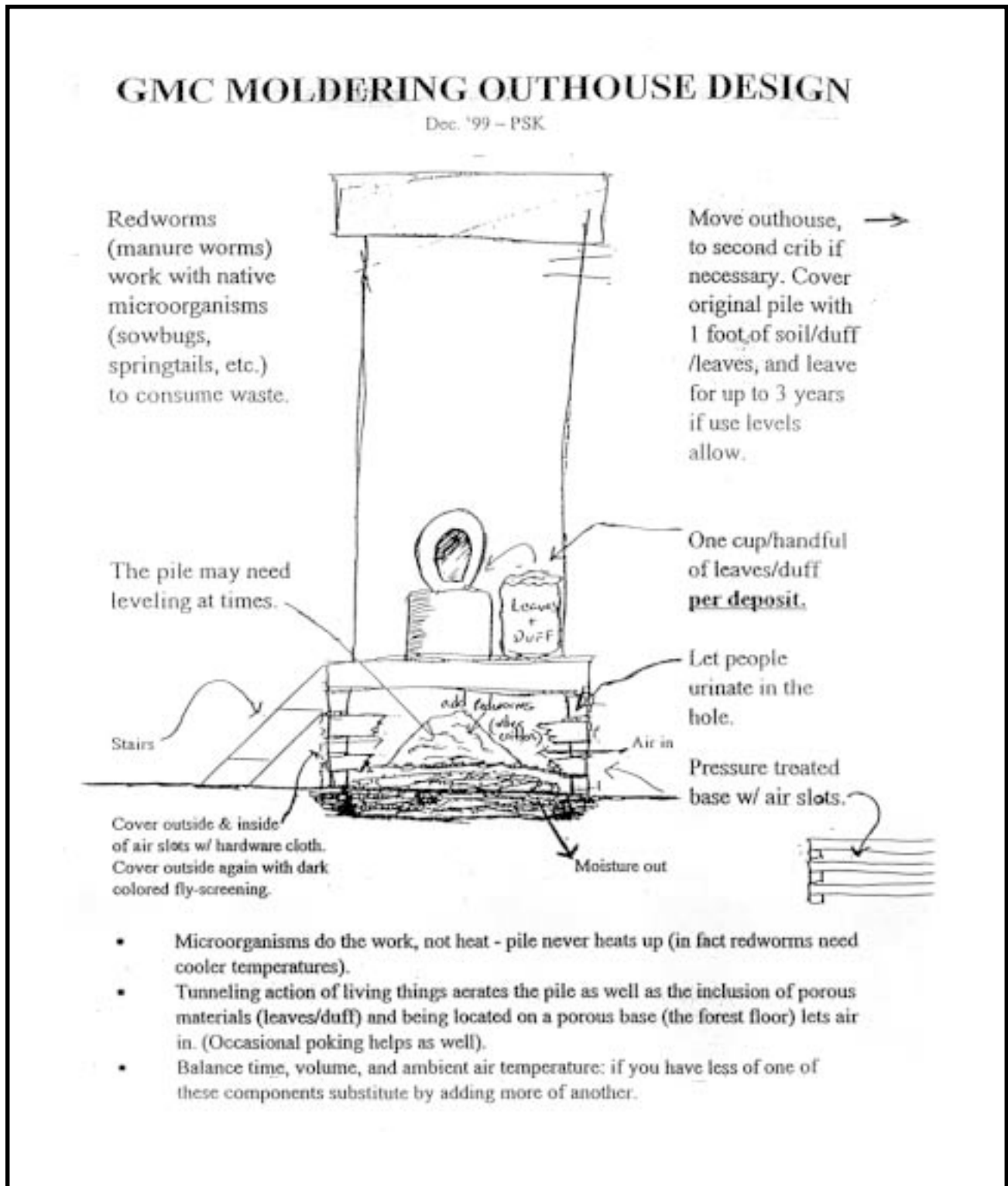
Figure 8.1—Conceptual diagram for the Green Mountain Club moldering privy. Not to scale. This diagram shows only one composting chamber. Current Green Mountain Club design utilizes a double-chambered system. When one chamber is full in the new design, it is capped with a lid, and the outhouse building is shifted over the empty chamber.” Drawing from Lars Botzjorns, Pete Ketcham, and the Green Mountain Club.
