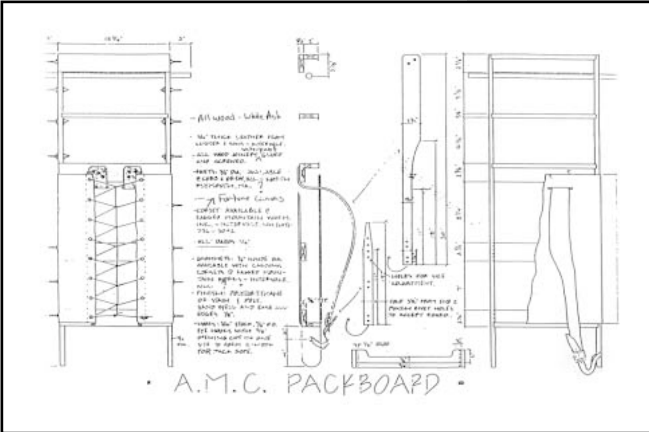
Figure P.3—Plans for construction of the Appalachian Mountain Club's wooden packboard. This packboard has been found to be the best for transporting composting toilet system components into the field as well as bark mulch or other bulking agents by the Green Mountain Club and Appalachian Mountain Club.
