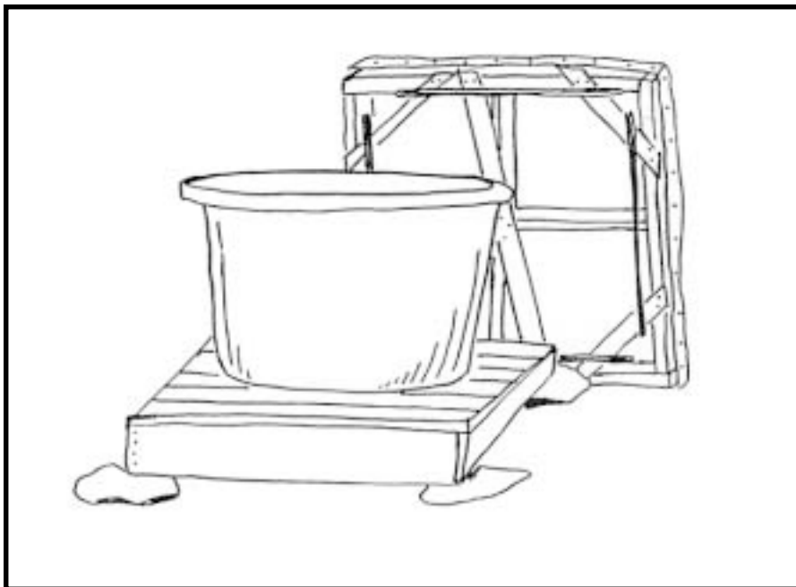
Figure 9.2—Diagram depicting the Green Mountain Club batch-bin compost system bin and lid. The lid is constructed of dimensional lumber. The Green Mountain Club recommends using manufactured plastic lids whenever possible because they have a longer life expectancy in the field and are less likely to leak. If cost is a factor, a wooden lid may be the best option. Diagram from the Green Mountain Club.”
