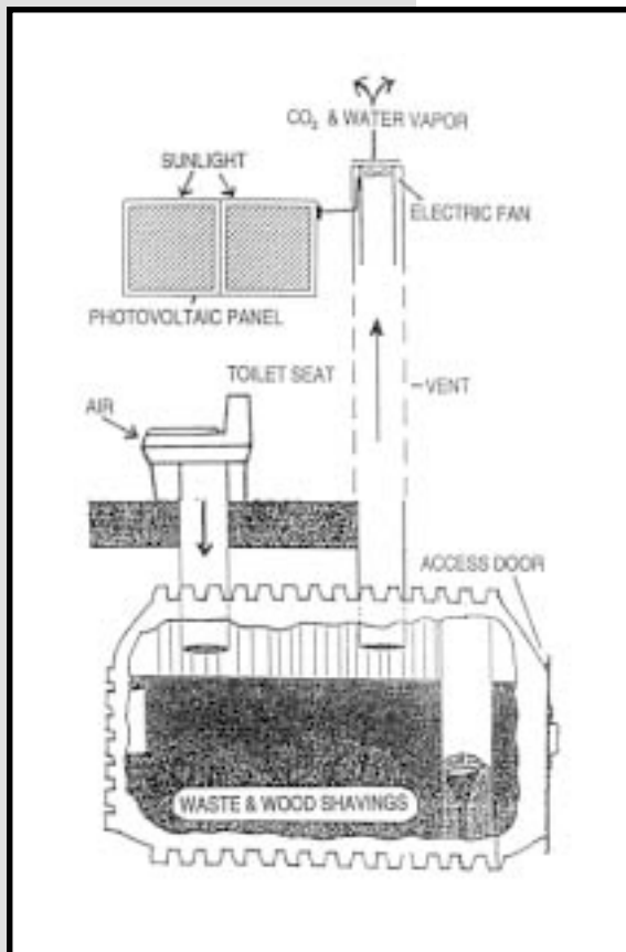
Figure 11.2—A cutaway view of a Bio-Sun WRS 1000, the model installed at the Randolph Mountain Club's Gray Knob Cabin in the northern Presidential Range of the White Mountains in New Hampshire. Note that the bottom of the tank does not slope. Aged compost must be raked towards the rear access door by the operator, and newer waste must be pushed forward. Schematic from Bio-Sun Systems, Inc. and the Randolph Mountain Club.
