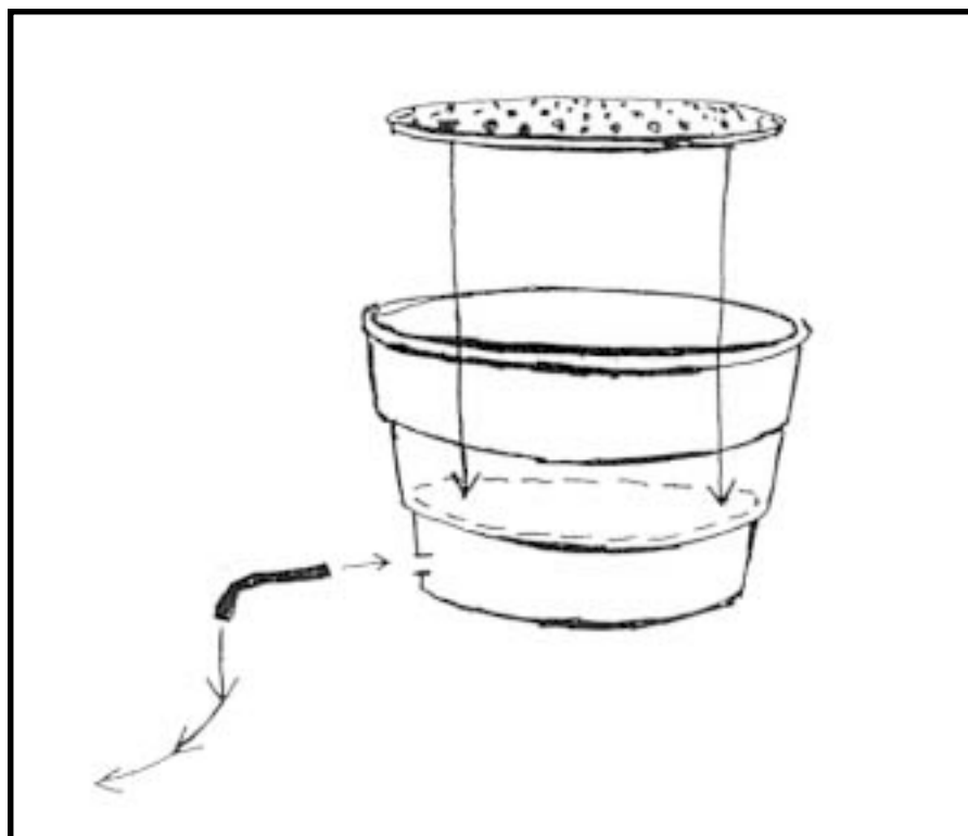
Figure 10.2—Diagram illustrating the placement of a perforated stainless-steel strainer plate in a 70-gallon sewage catcher. This is the first step to attaching a beyond-the-bin liquid management system. The hose leads liquid away for treatment. Diagram from the Appalachian Mountain Club Trails Department.”
