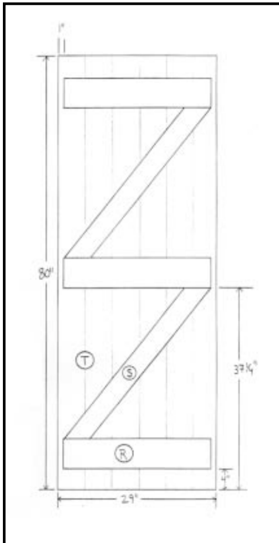
Figure H.1—Plans for a lightweight outhouse. It can be used with a moldering privy, or with a batch-bin or beyond-the-bin system when placed over a vault to hold the catcher (see Chapter 7, the Batch-Bin System). This plan does not show a lift-up bench seat or a rear access door, either of which makes it more convenient to inspect and manipulate the waste pile. Plans from Jeff Bostwick, Green Mountain Club.
