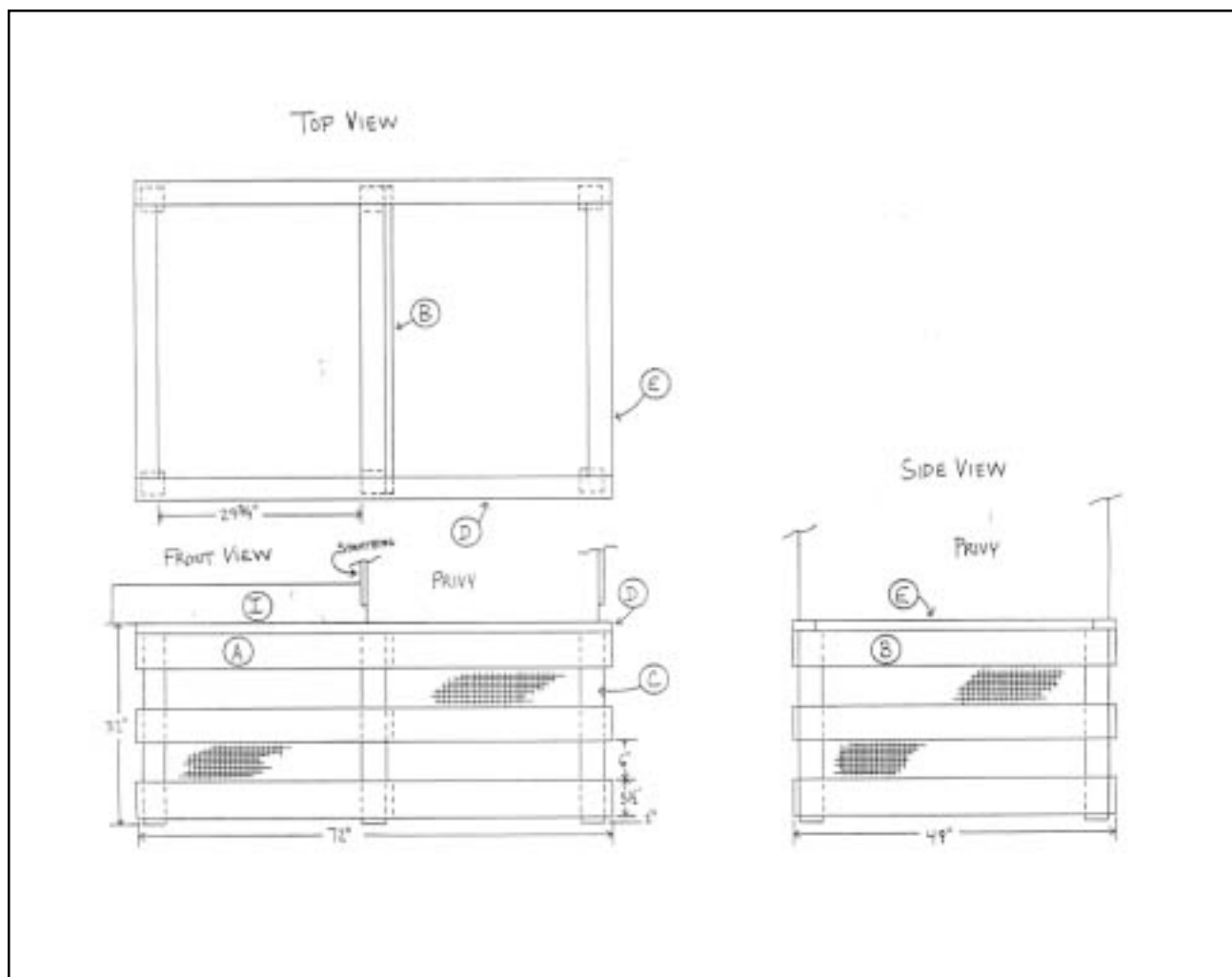
Figure I.1—Plans for the construction of the latest prototype of the Green Mountain Club moldering privy, a double-chambered design. Plans from of Jeff Bostwick, Green Mountain Club.
