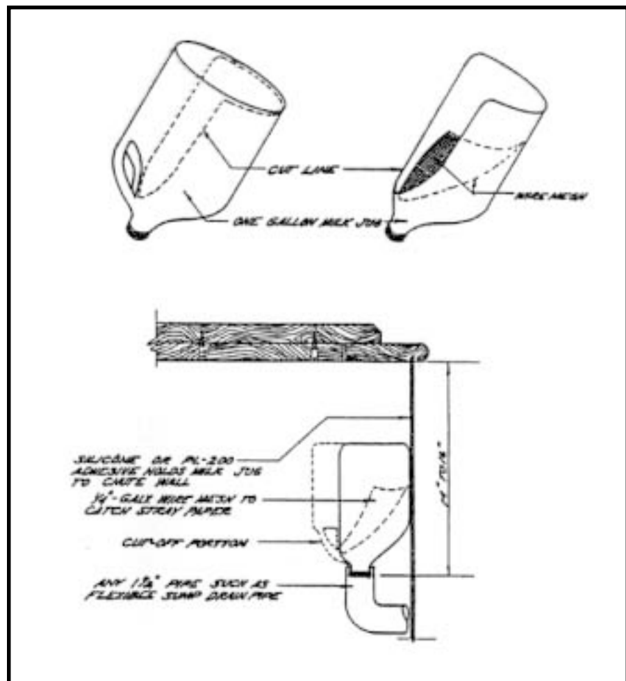
Figure 9.4—An example of a simple, home-made, urine diverting device that could have many applications with a variety of systems, both those described in this manual and others in use on the A.T. The drain pipe could lead to a beyond-the-bin liquid management system or a simple rock-lined dry well. State and local regulations may dictate how the liquid is managed." From The Composting Toilet System Book by David Del Porto and Carol Steinfeld.
